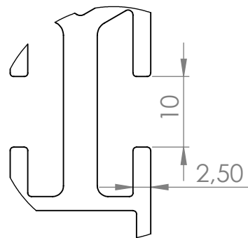
DETAIL A SCALE 4 : 3
